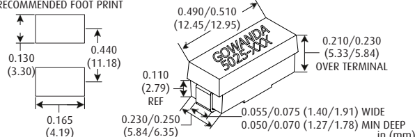
RECOMMENDED FOOT PRINT
