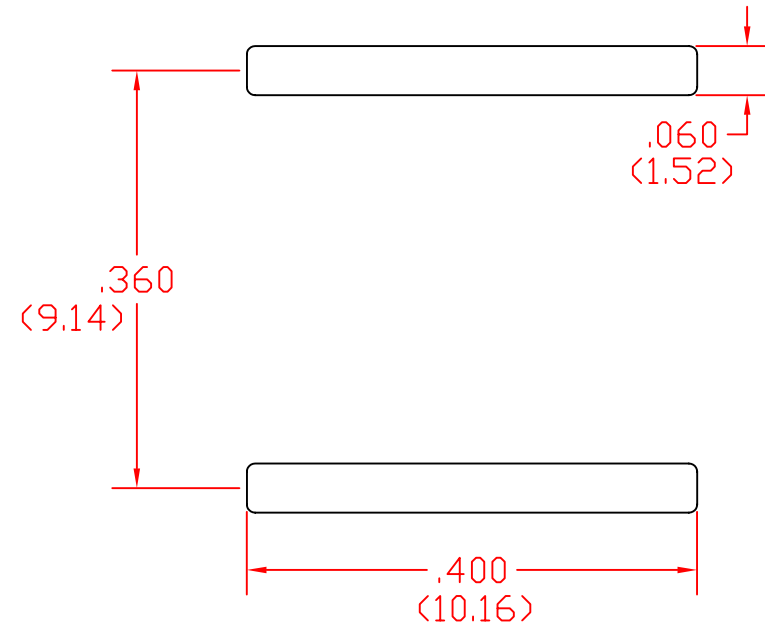
Recommended Foot Print
