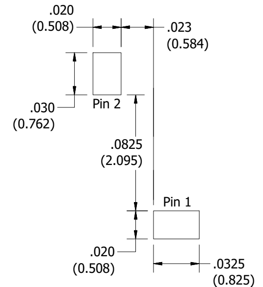
Recommended Footprint
