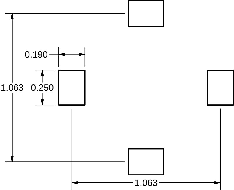
Recommended Foot Print
