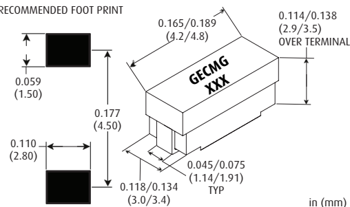
RECOMMENDED FOOT PRINT
