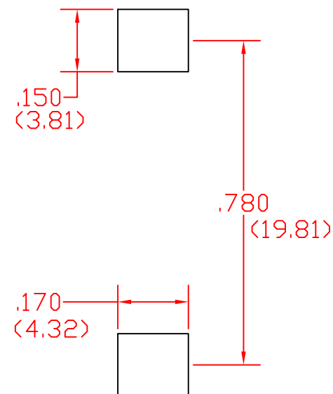
Recommended Foot Print
