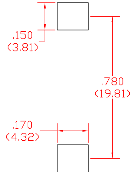
Recommended Foot Print
