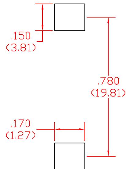
Recommended Foot Print
