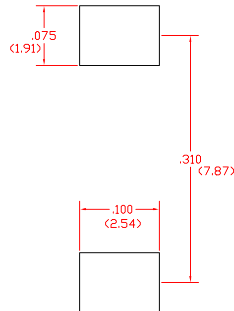
Recommended Foot Print
