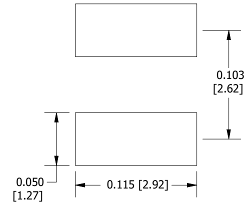
Recommended Footprint
