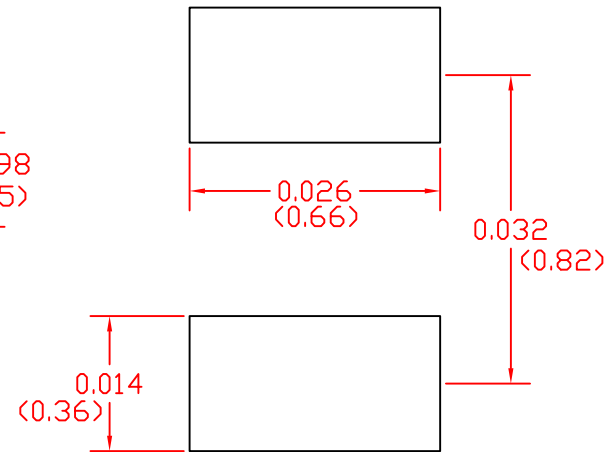
Recommended Foot Print
